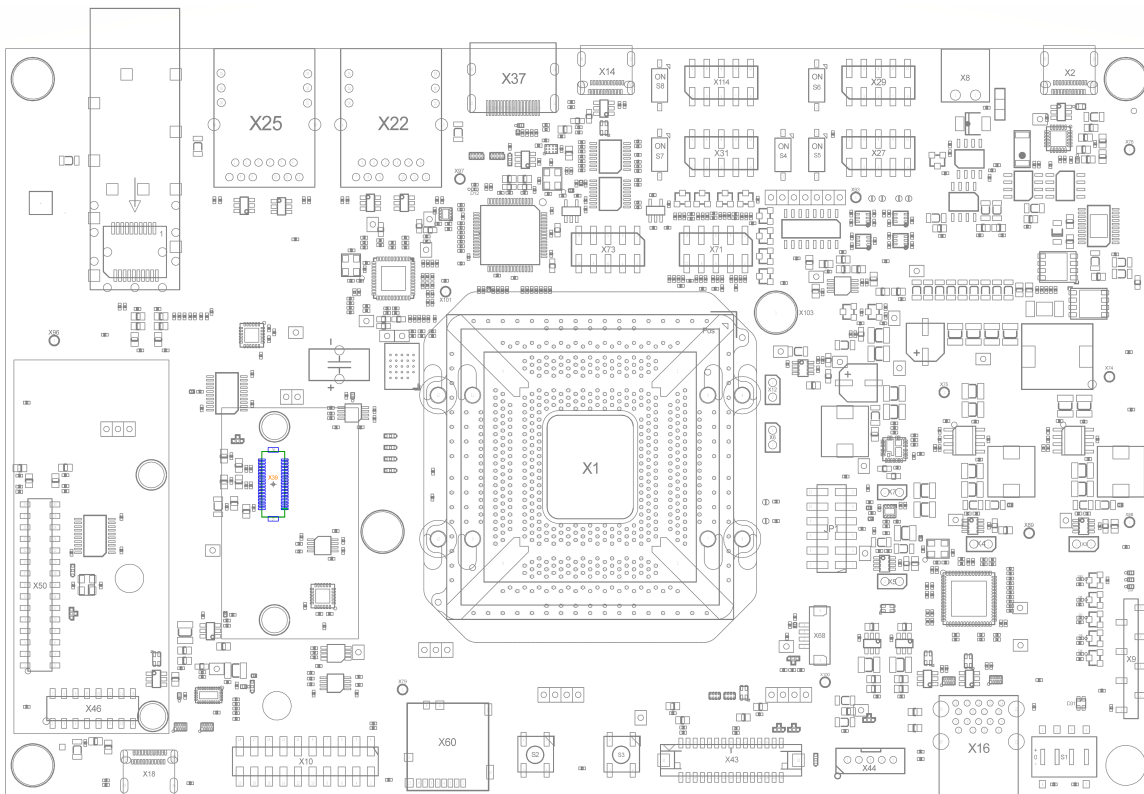
FIGURE 30: MIPI-DSI (X39)
