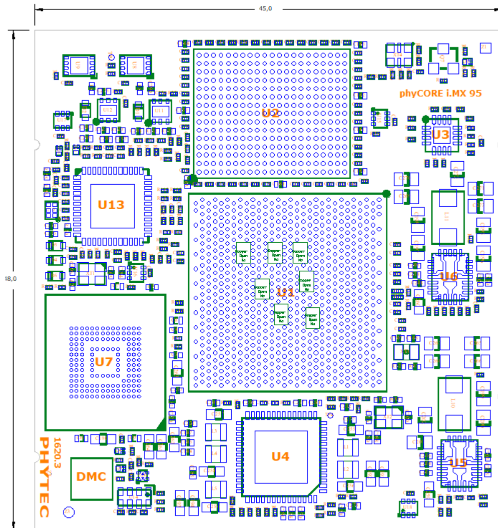
FIGURE 6: phyFLEX-i.MX 95 FPSC Footprint (top to bottom view; unit in mm)
