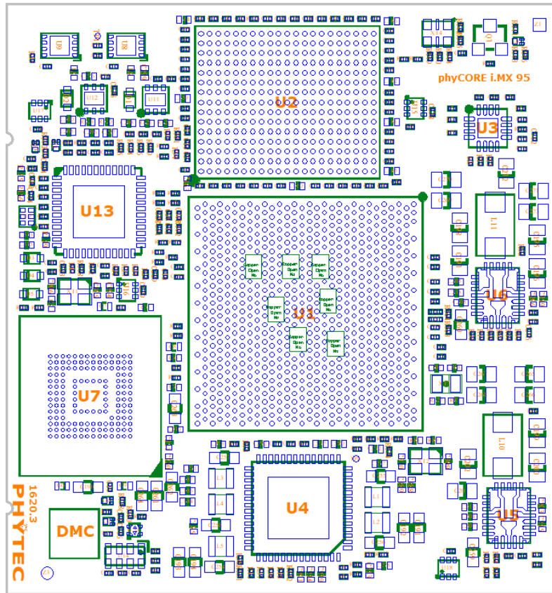
FIGURE 2: phyFLEX-i.MX 95 Component Placement (1620.3 Top View)
