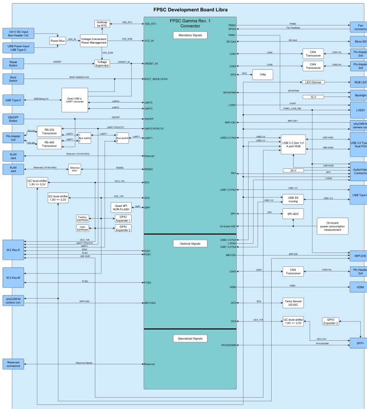
FIGURE 8: Libra Development Board Block Diagram
