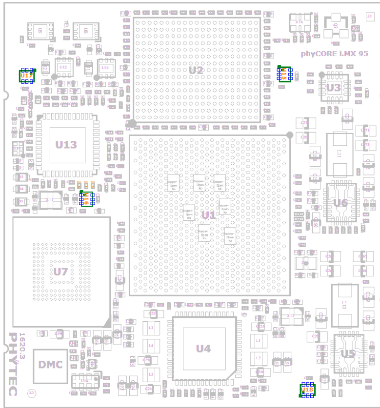
FIGURE 5: Temperature Sensor Locations
