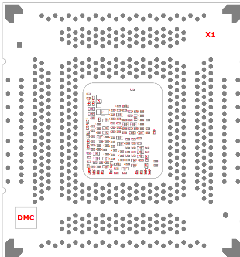
FIGURE 3: phyFLEX-i.MX 95 Component Placement (1620.3 Bottom View)
