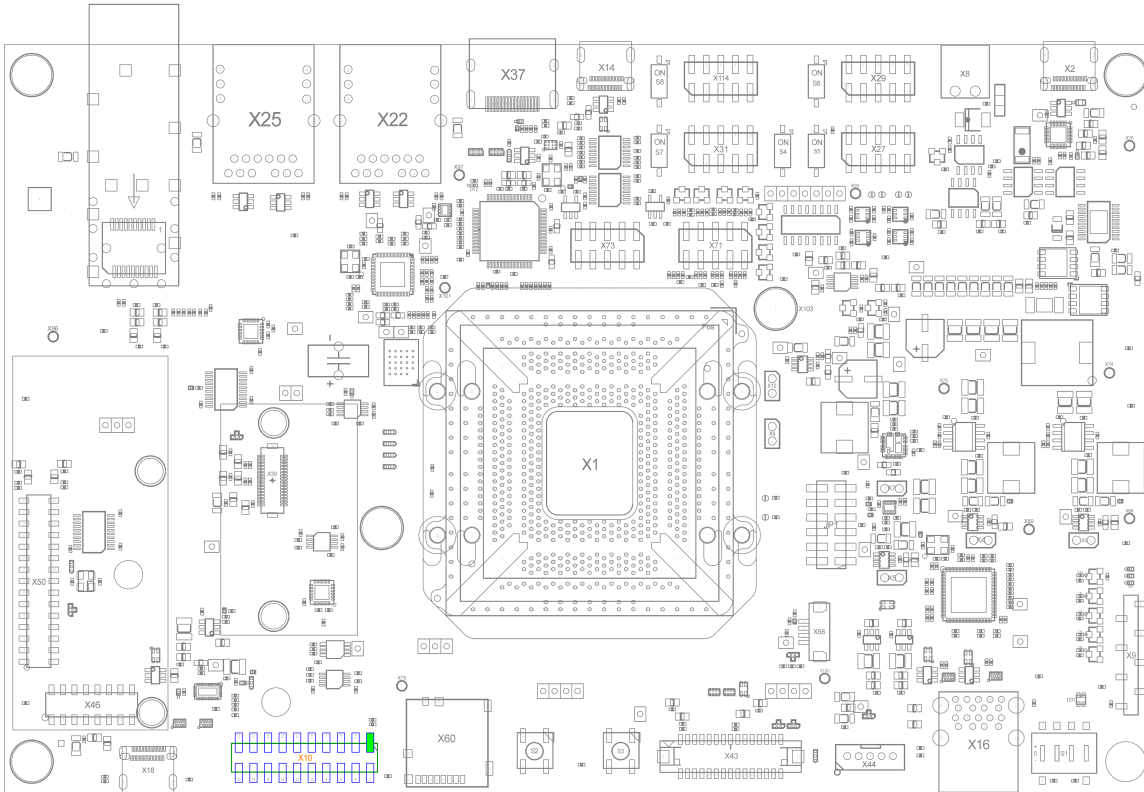
FIGURE 32: JTAG (X10)
