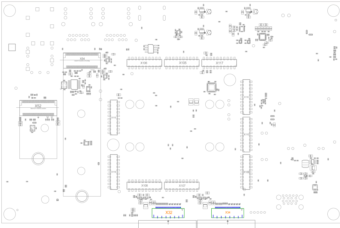
FIGURE 26: phyCAM-M MIPI CSI-2 Camera Connectors (X32/X34)
