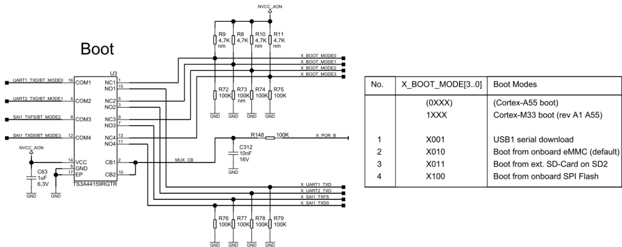
FIGURE 4: phyFLEX-i.MX 95 FPSC Onboard Boot Configuration Schematic
