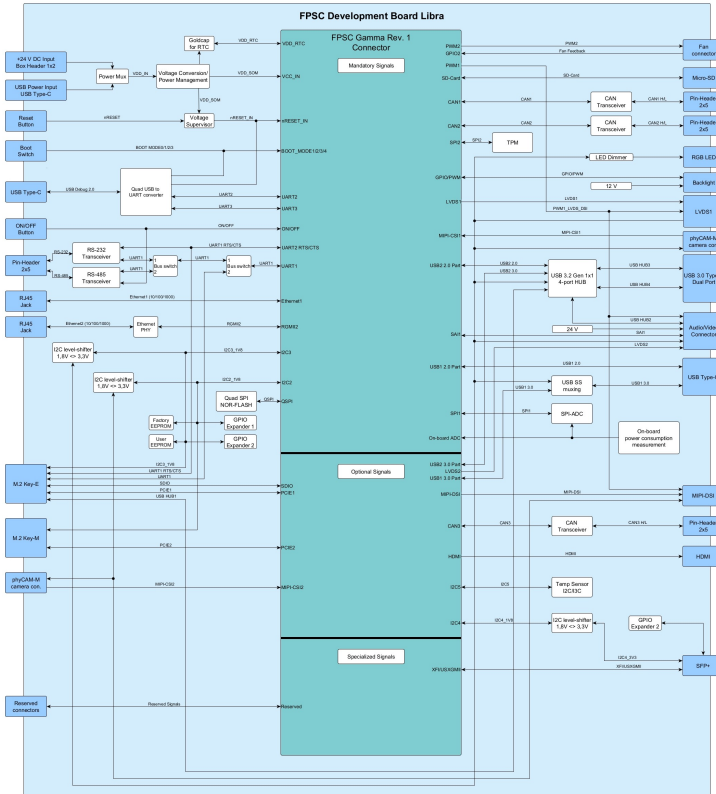
FIGURE 6: Libra Development Board Block Diagram
