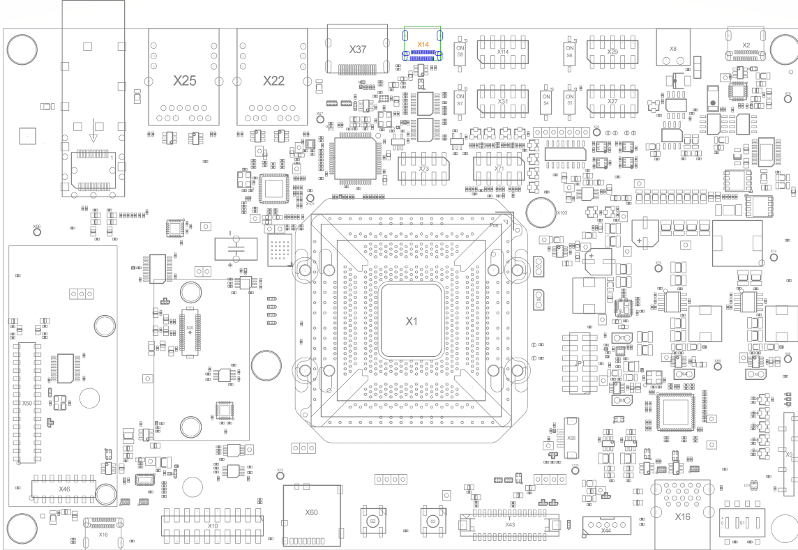
FIGURE 20: USB Debug Connector (X14)
