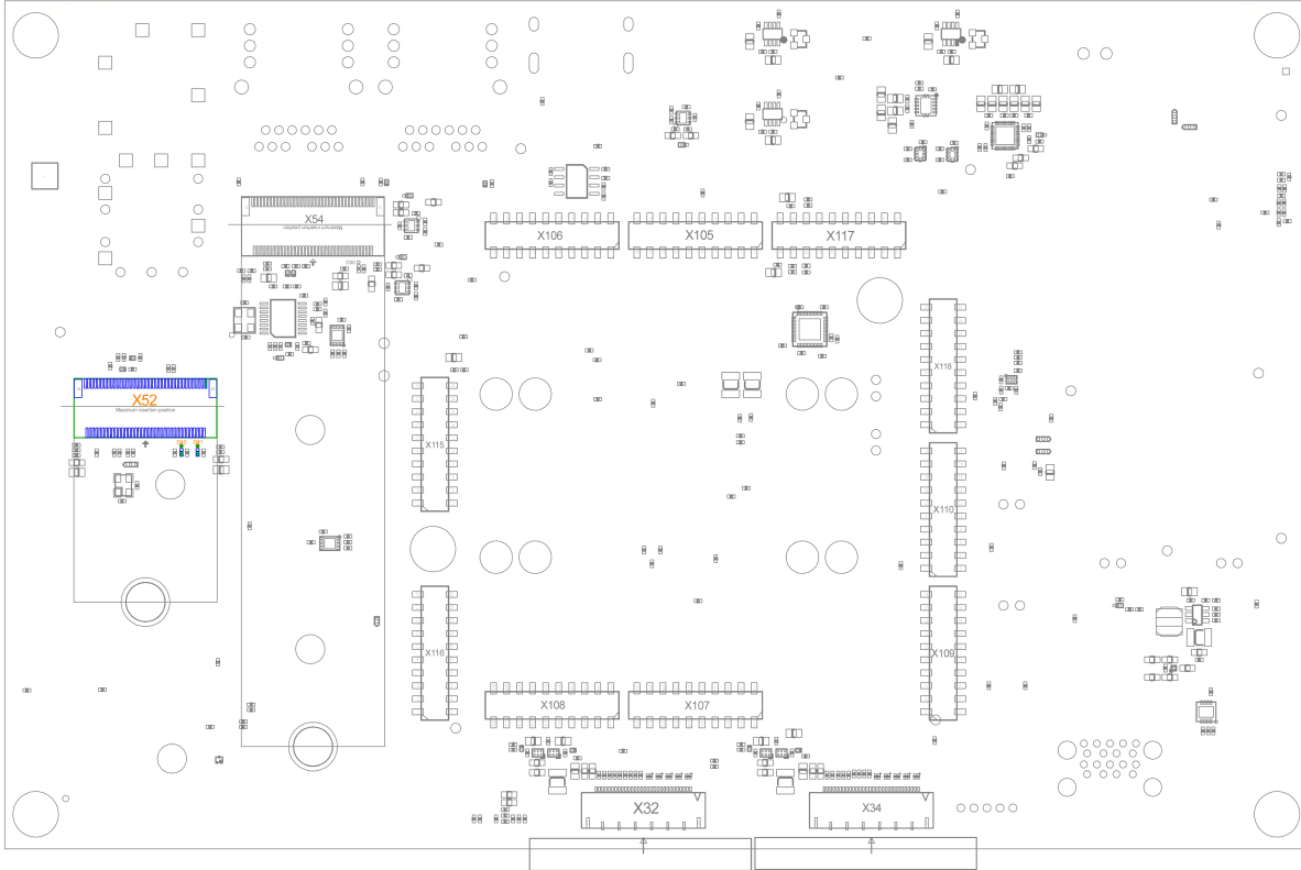
FIGURE 22: M.2 Key-E Connector (X52)
