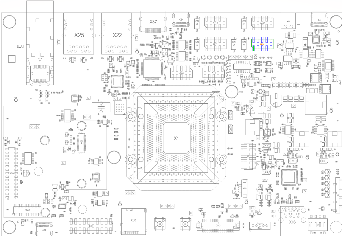
FIGURE 15: RS-232 and RS-485 Connector (X27)
