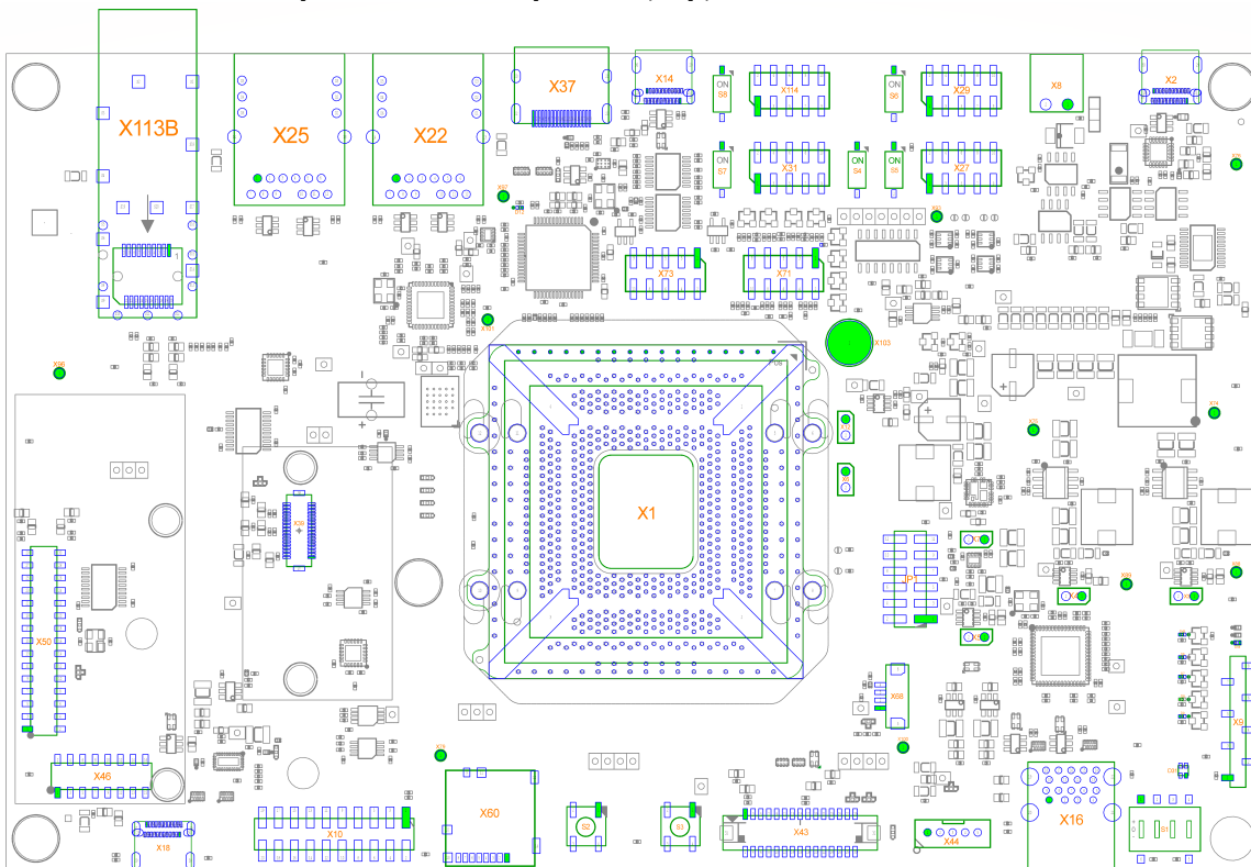
FIGURE 7: Libra Development Board Components (Top)
