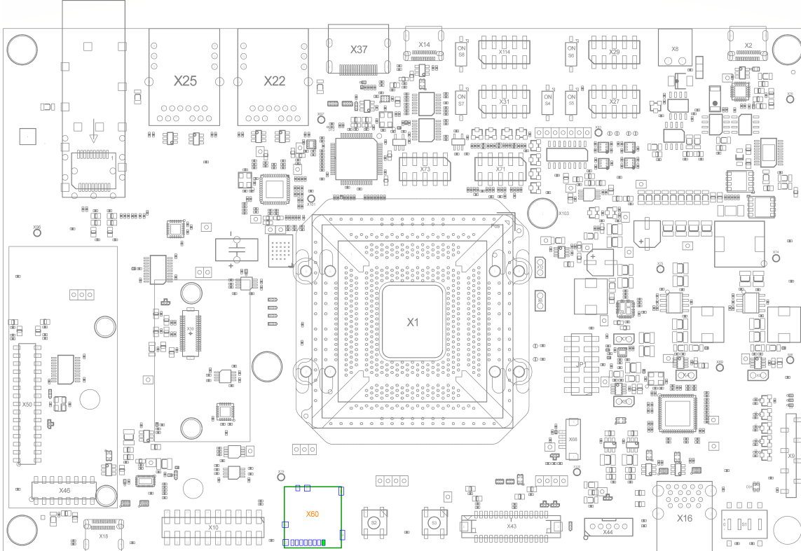
FIGURE 21: SD / MM Card Connector (X60)
