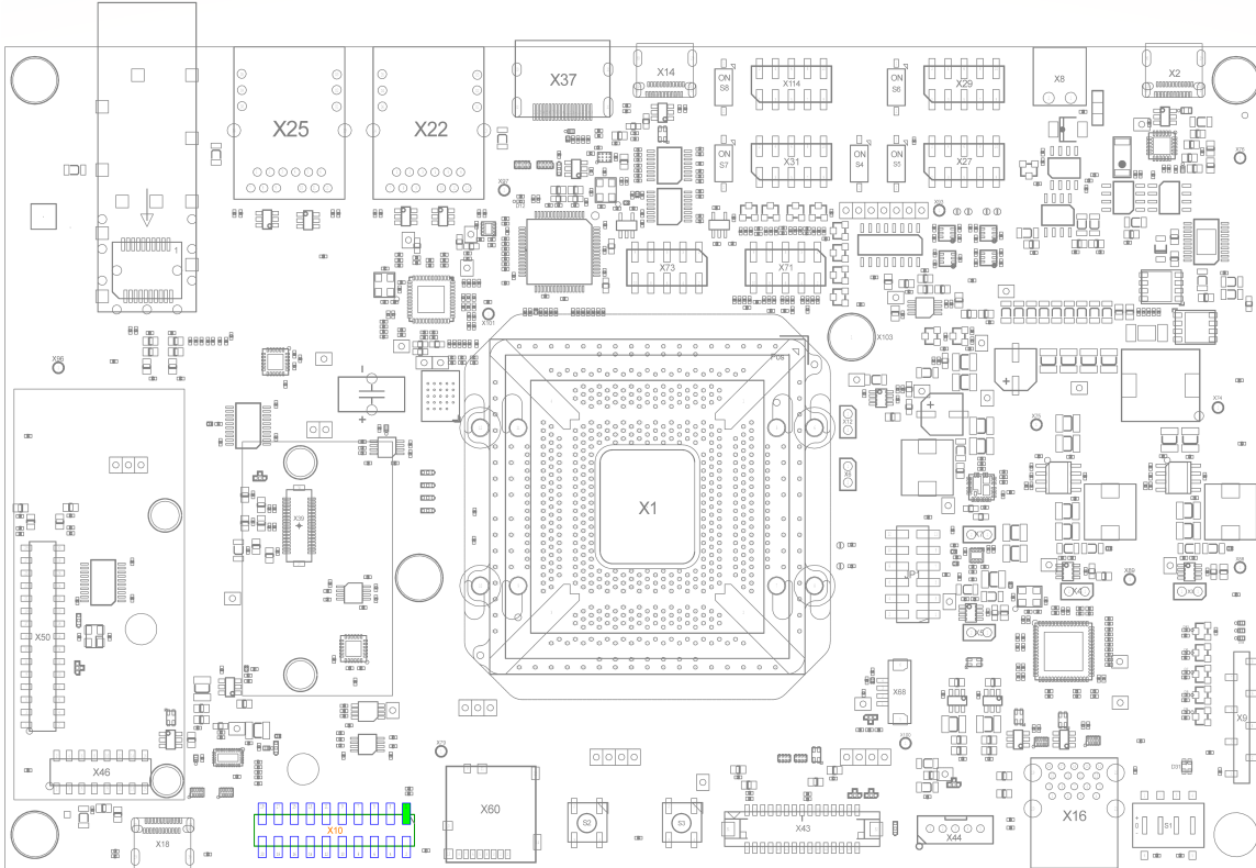
FIGURE 30: JTAG (X10)
