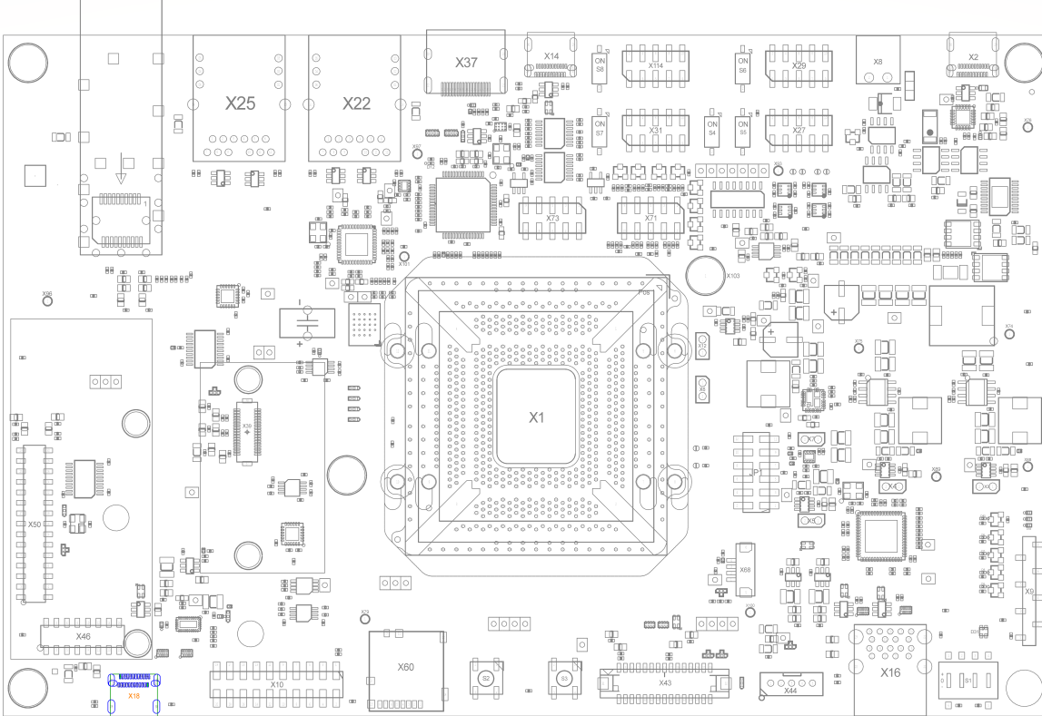
FIGURE 19: USB 3.2 Gen1 Connector (X18)
