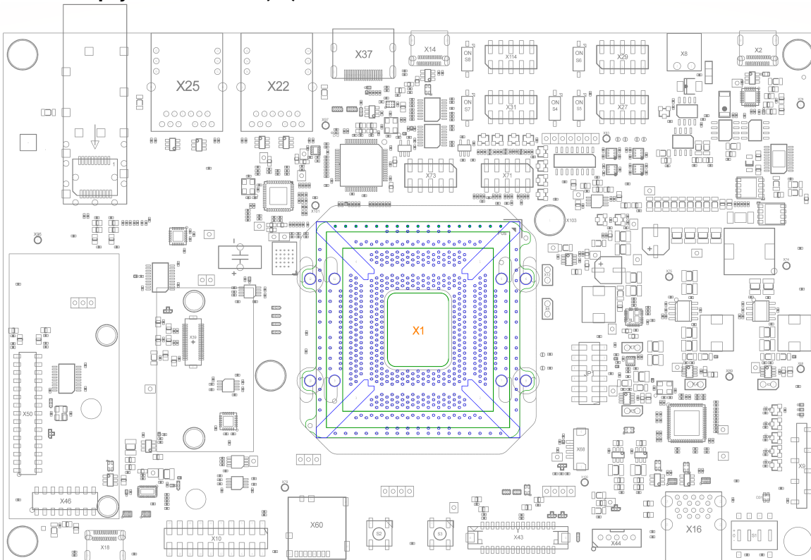
FIGURE 13: phyFLEX Connector (X1)
