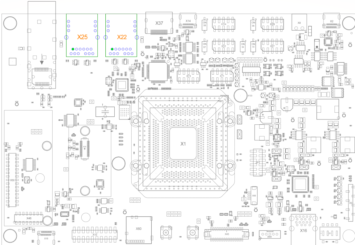
FIGURE 17: Ethernet Connectors (X22/X25)
