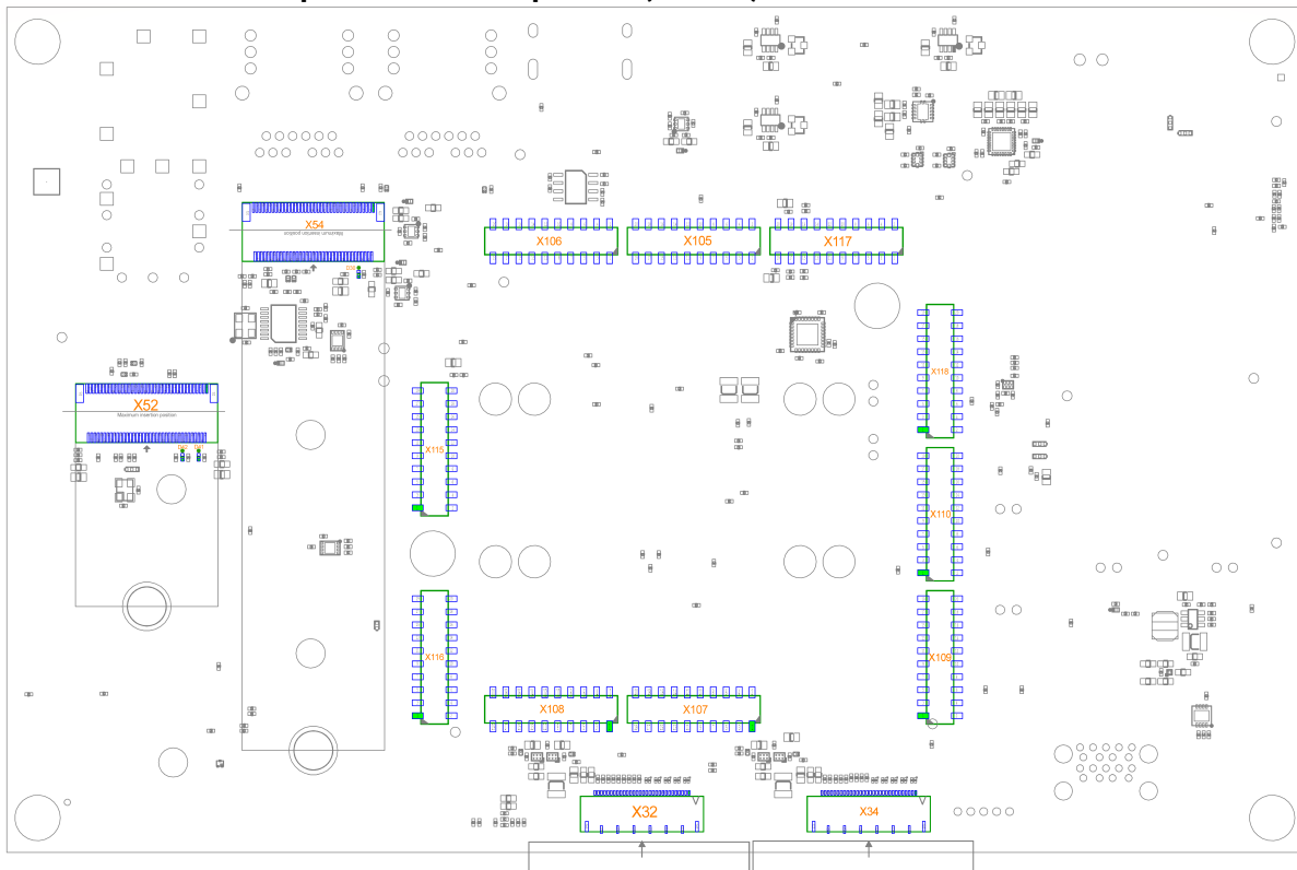
FIGURE 8: Libra Development Board Components (Bottom)
