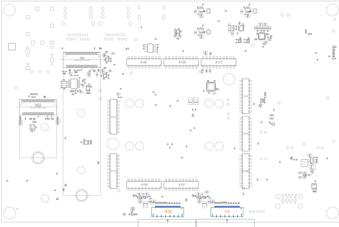
FIGURE 24: phyCAM-M MIPI CSI-2 Camera Connectors (X32/X34)
