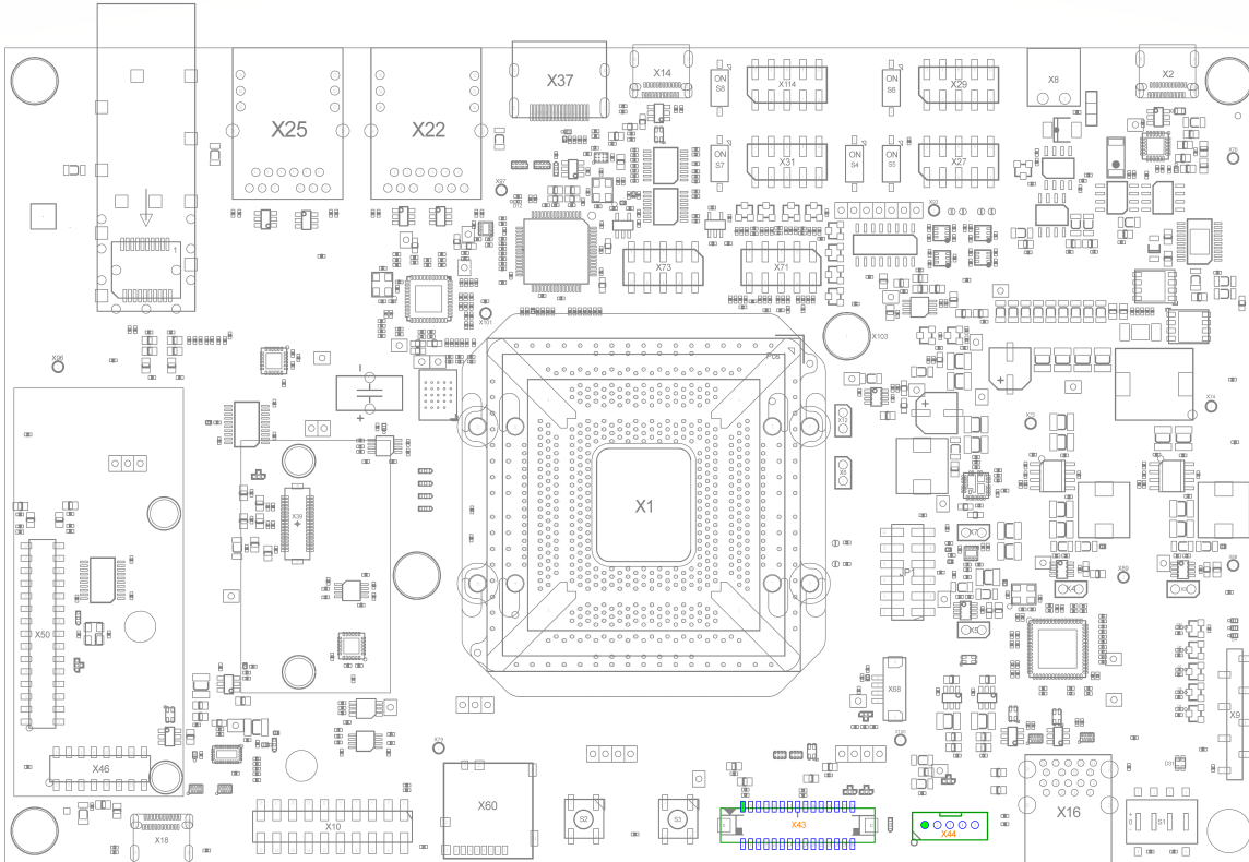
FIGURE 27: LVDS1 Connectors (X43/X44)
