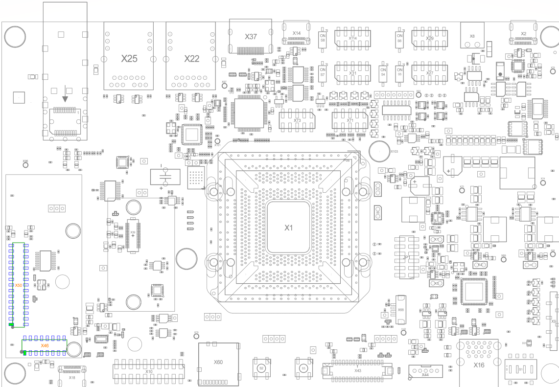
FIGURE 26: Audio/Video Connectors (X46/X50)
