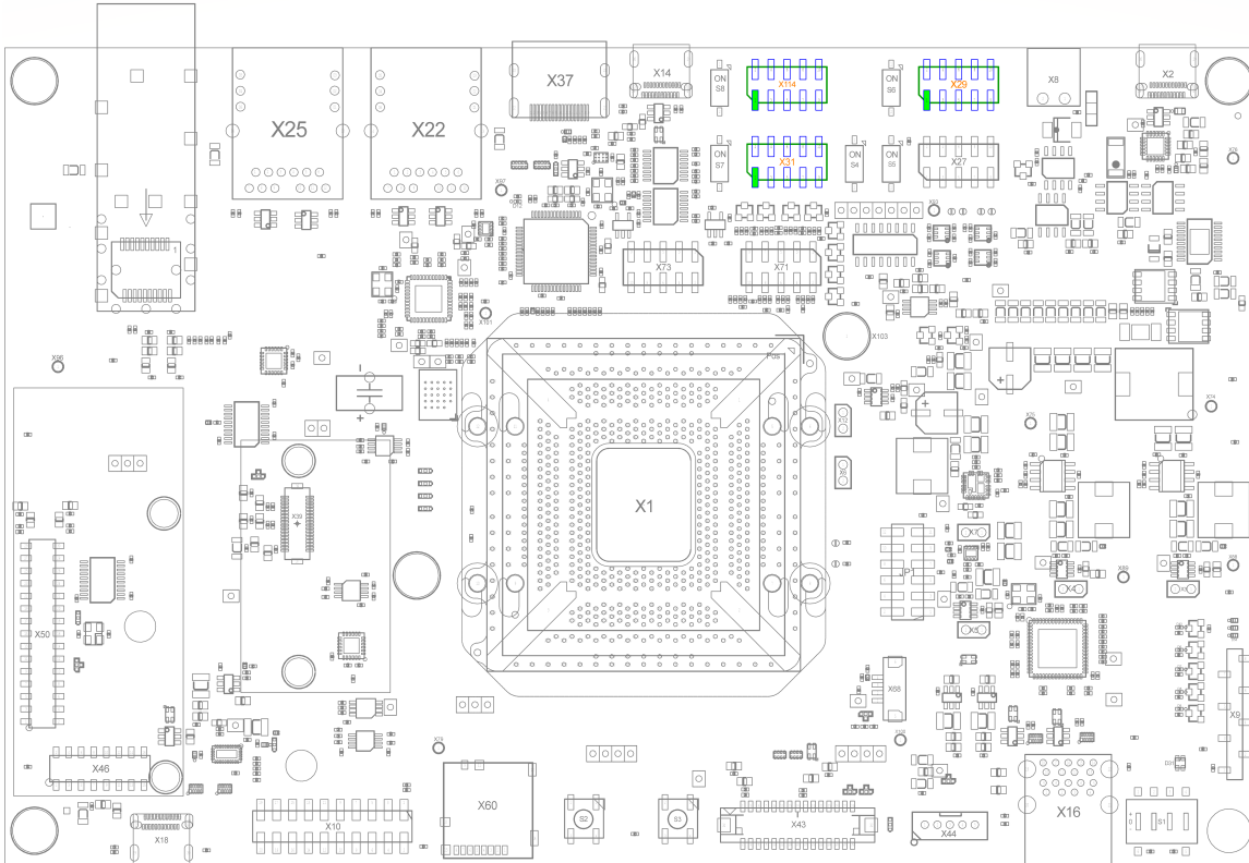
FIGURE 16: CAN FD (X29/X31/X114)
