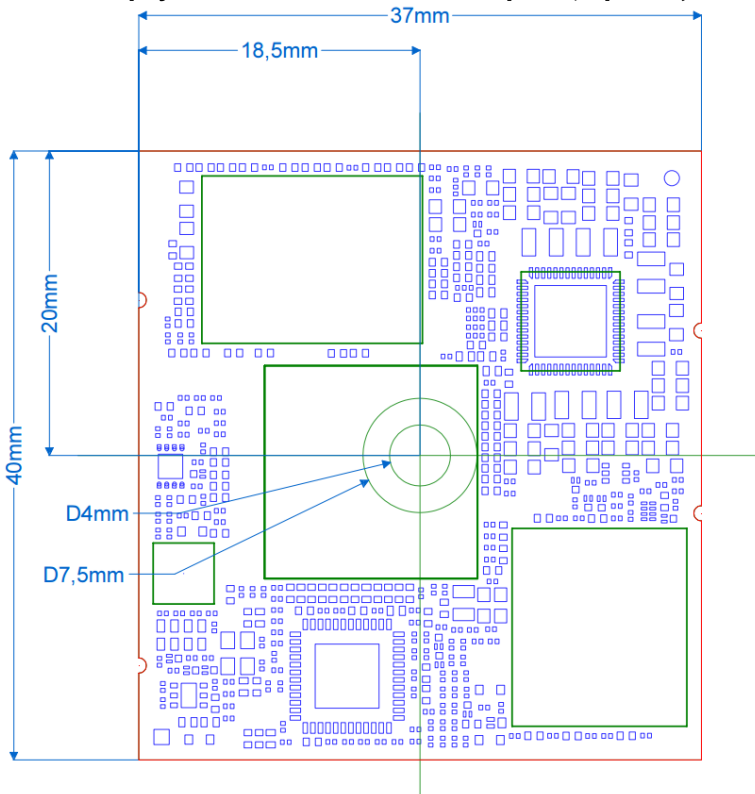
FIGURE 5: phyFLEX-STM32MP2x FPSC Footprint (top view; unit in mm)
