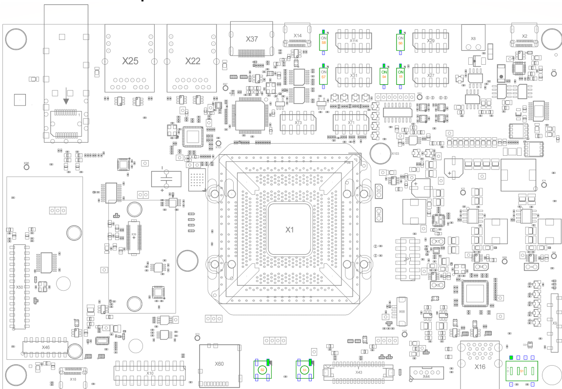
FIGURE 11: Libra Development Board Switch Locations
