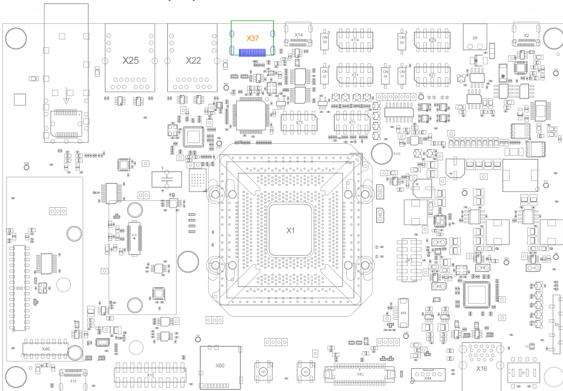
FIGURE 25: HDMI Connector (X37)
