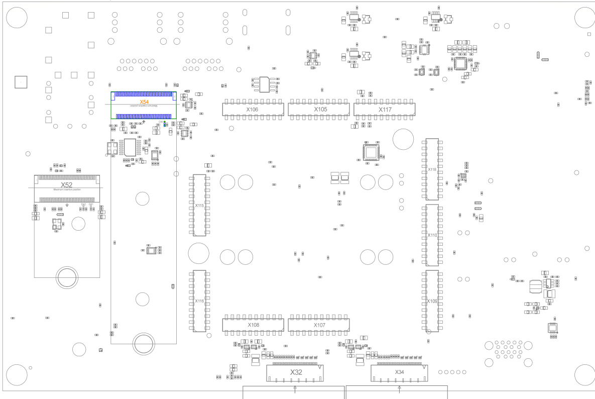
FIGURE 23: M.2 Key-M (X54)
