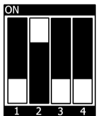
Figure 1: Boot Mode DIP Switch (S3) SD Card Setting
