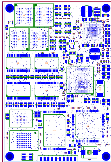
PCM 637 phyCORE-IMX31
