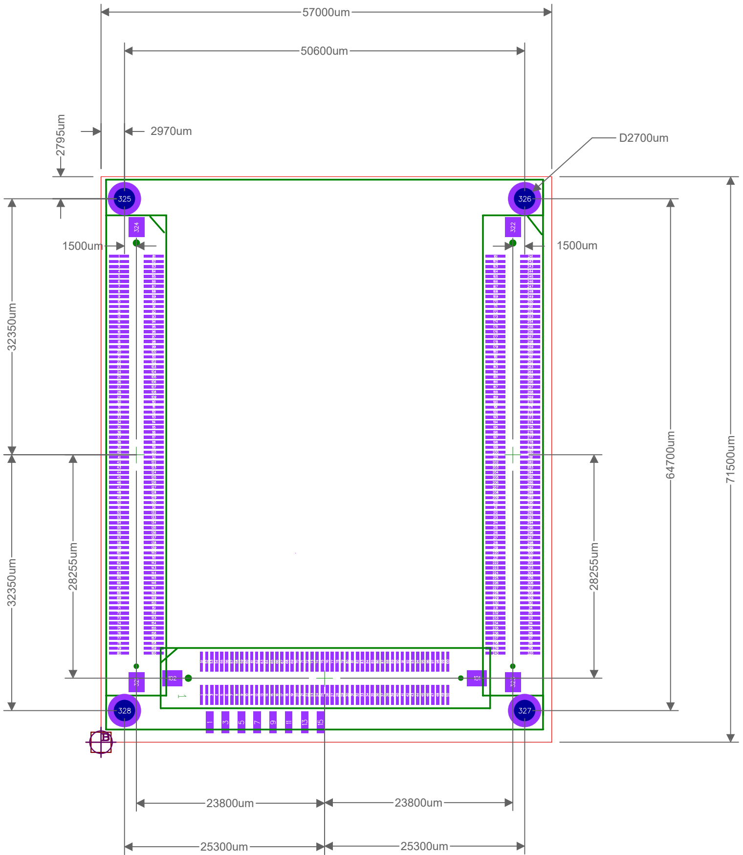
Top View, connectors on bottom side
