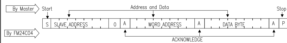
Figure 5 Byte Write
