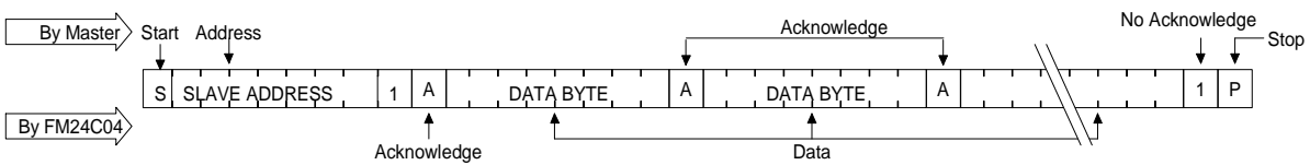
Figure 8 Sequential Read
