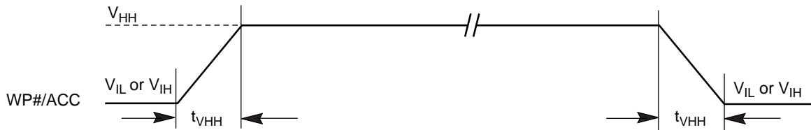
Figure 23. Accelerated Program Timing Diagram
