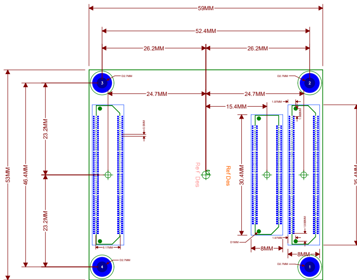
Pad size: 0,3 x 1,45mm Plated hole size: 5mm and 2,7mm hole
