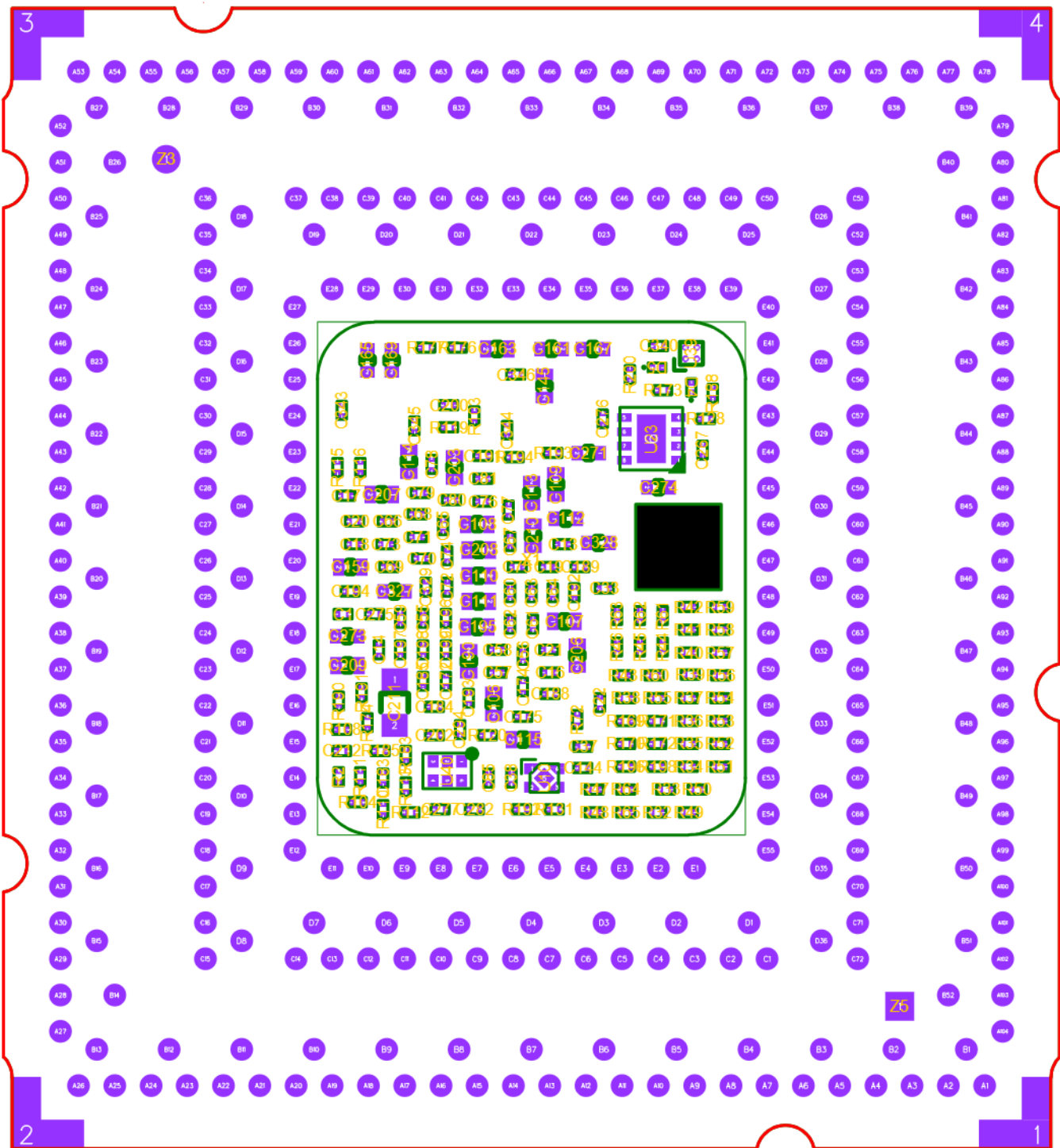
phyCORE-i.MX8M Mini 1518.3a Component Placement Diagram (Backside)
