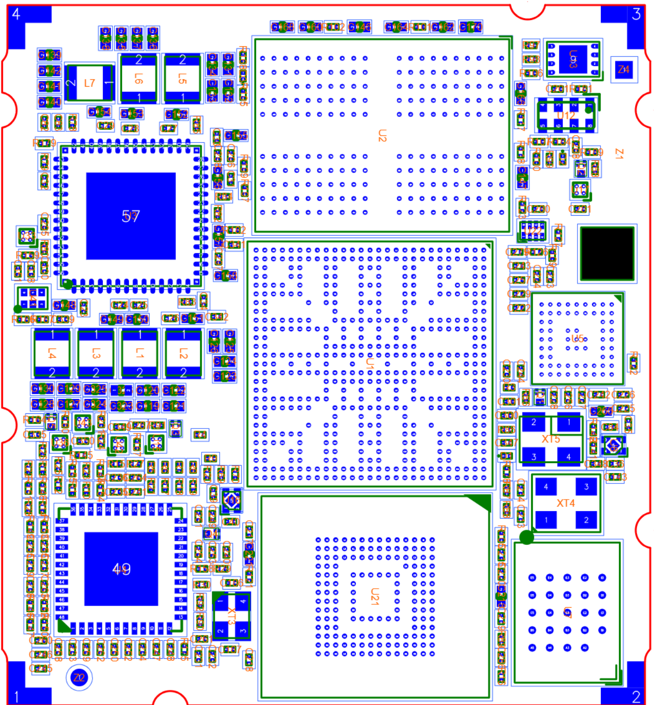
phyCORE-i.MX8M Mini 1518.3a Component Placement Diagram (Frontside)
