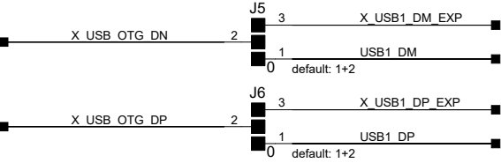
Jumper for USB1 OTG on micro USB or expansion connector
