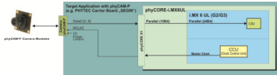
figure 3: Block Diagram of a phyCAM-P solution with phyCORE-i.MX6UL (G2 / G3) and the go out on the phyBOARD-SEGIN-i.MX6UL - SBC
